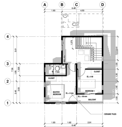
3 SECOND FLOOR PLAN A-1 1:75
