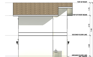
6 REAR ELEVATION A-1 1:75
