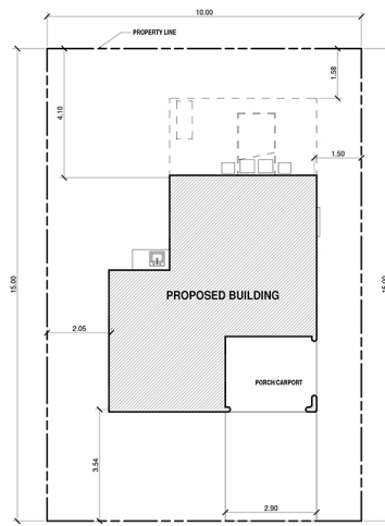
1 SITE DEVELOPMENT PLAN A-1 1:75
