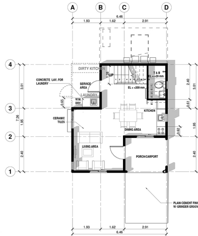
2 GROUND FLOOR PLAN A-1 1:75
