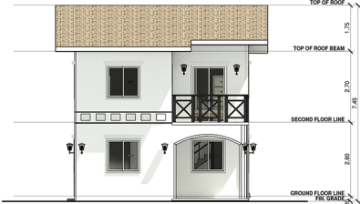
4 FRONT ELEVATION A-1 1:75
